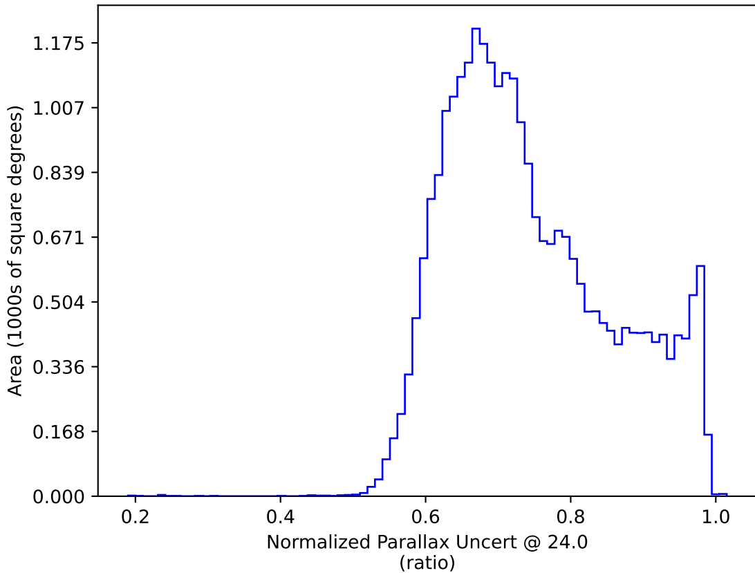
weather_cloudso18v3.4_10yrs All sky: Normalized Parallax Uncert @ 24.0
