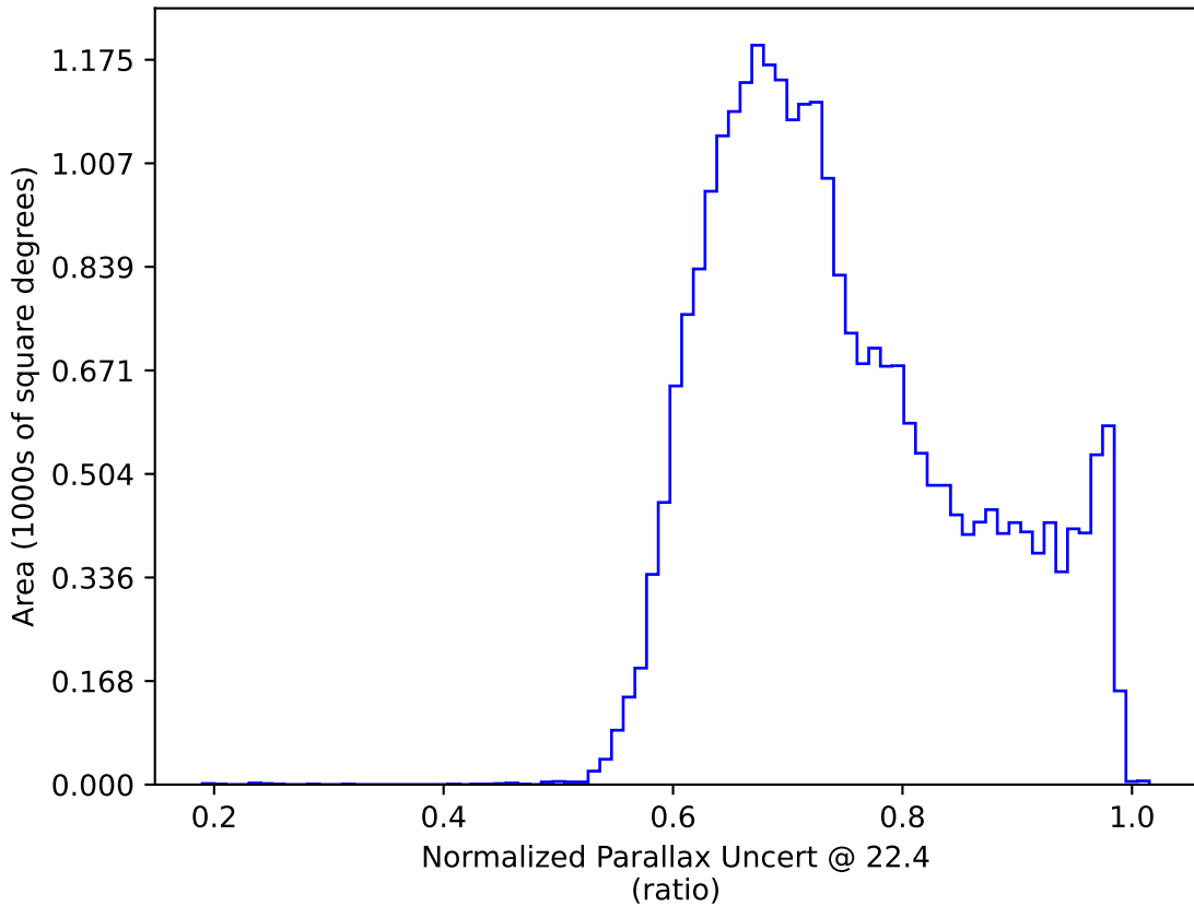
weather_cloudso18v3.4_10yrs All sky: Normalized Parallax Uncert @ 22.4
