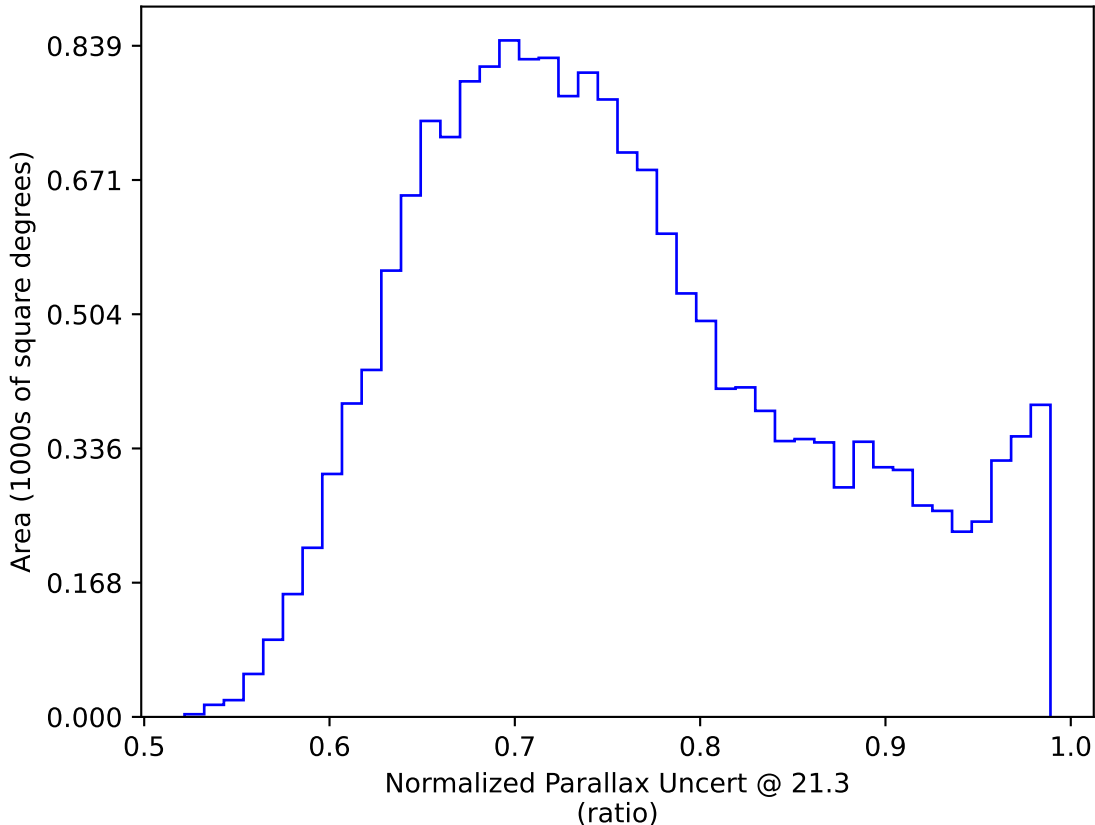
weather_cloudso18v3.4_10yrs WFD y band only: Normalized Parallax Uncert @ 21.3
