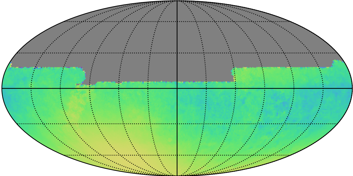
weather_cloudso18v3.4_10yrs All sky y band only: Normalized Parallax Uncert @ 21.3
