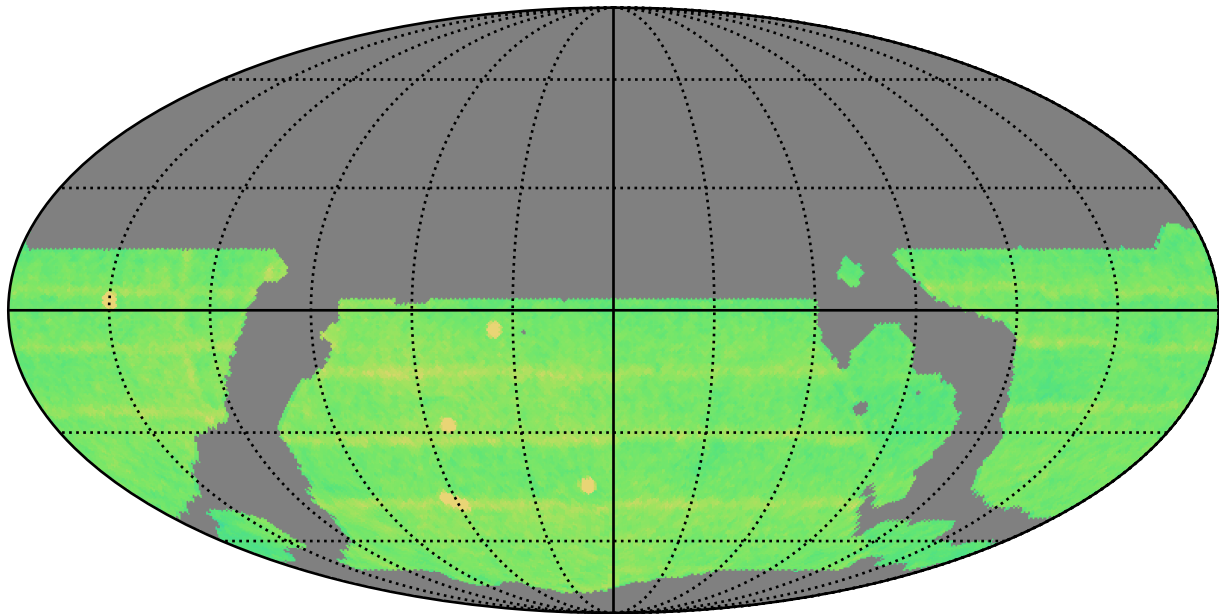
weather_cloudso18v3.4_10yrs WFD all bands: N Unique Nights
