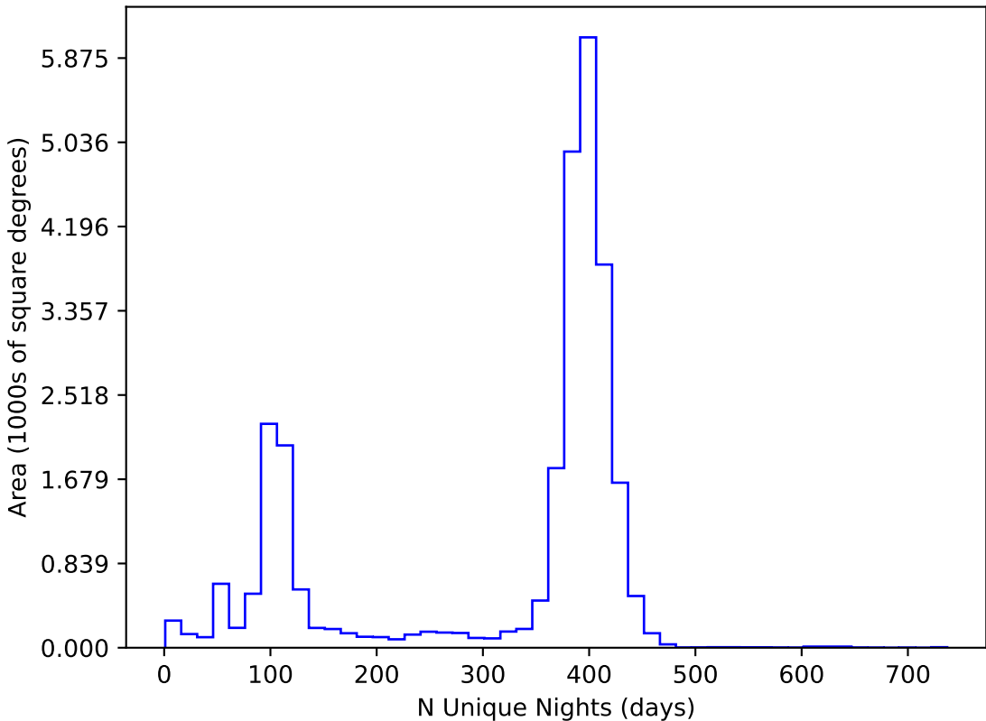
weather_cloudso18v3.4_10yrs All sky all bands: N Unique Nights
