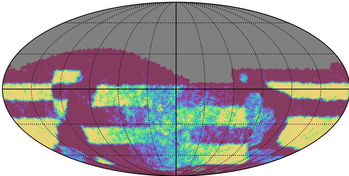
weather_cloudso18v3.4_10yrs Yr 3-4 z band: NVisits
