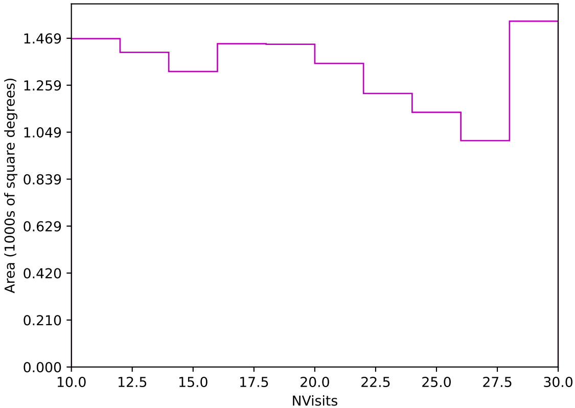
weather_cloudso18v3.4_10yrs Yr 3-4 z band: NVisits
