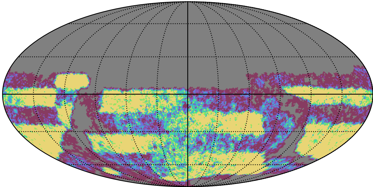
weather_cloudso18v3.4_10yrs Yr 3-4 u band: NVisits
