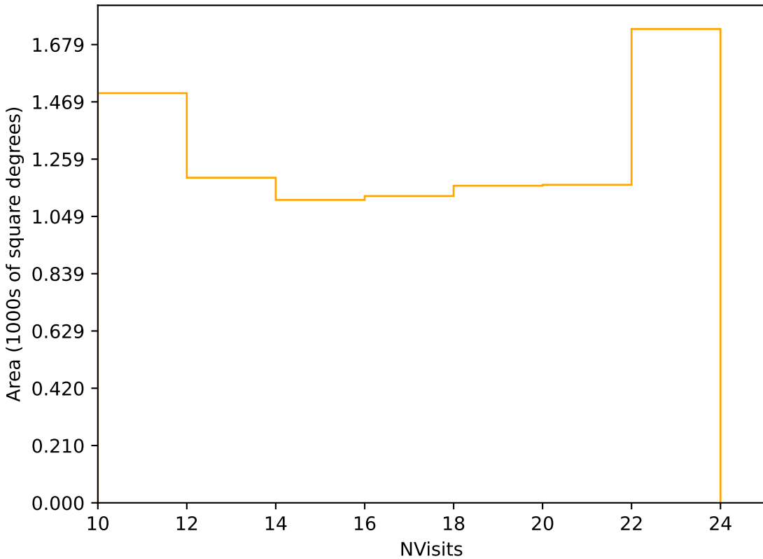
weather_cloudso18v3.4_10yrs Yr 3-4 r band: NVisits
