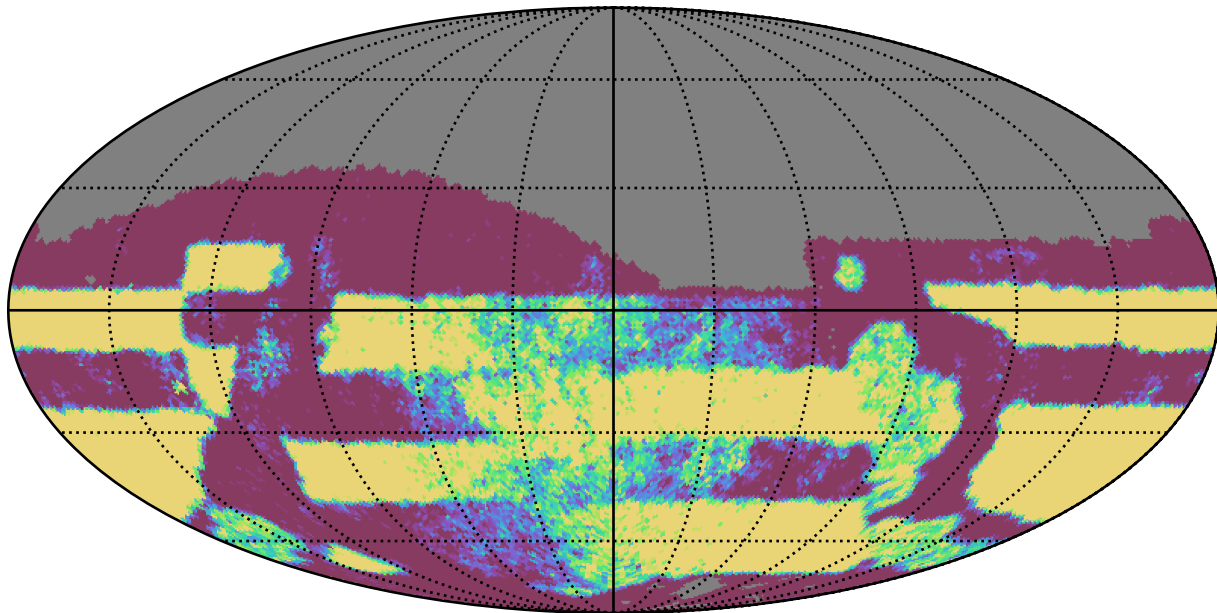
weather_cloudso18v3.4_10yrs Yr 3-4 i band: NVisits
