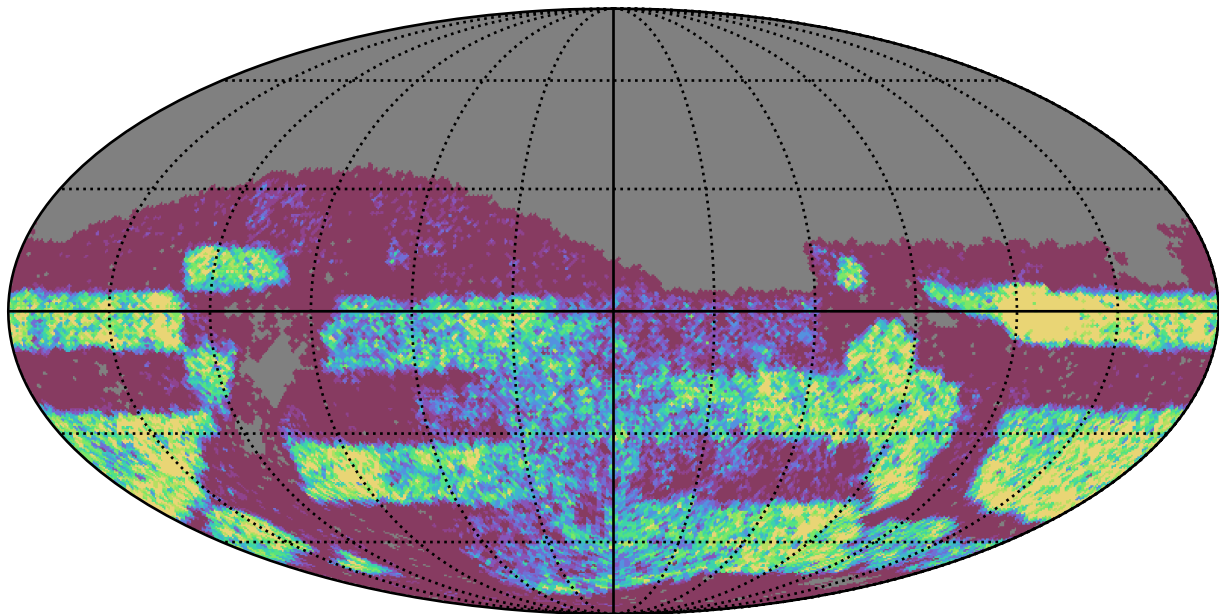
weather_cloudso18v3.4_10yrs Yr 3-4 g band: NVisits
