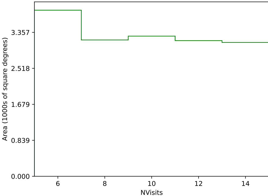
weather_cloudso18v3.4_10yrs Yr 3-4 g band: NVisits
