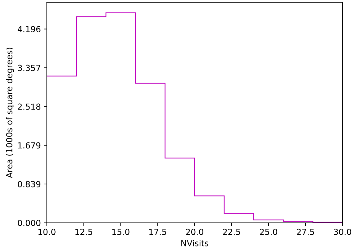
weather_cloudso18v3.4_10yrs Yr 1 z band: NVisits
