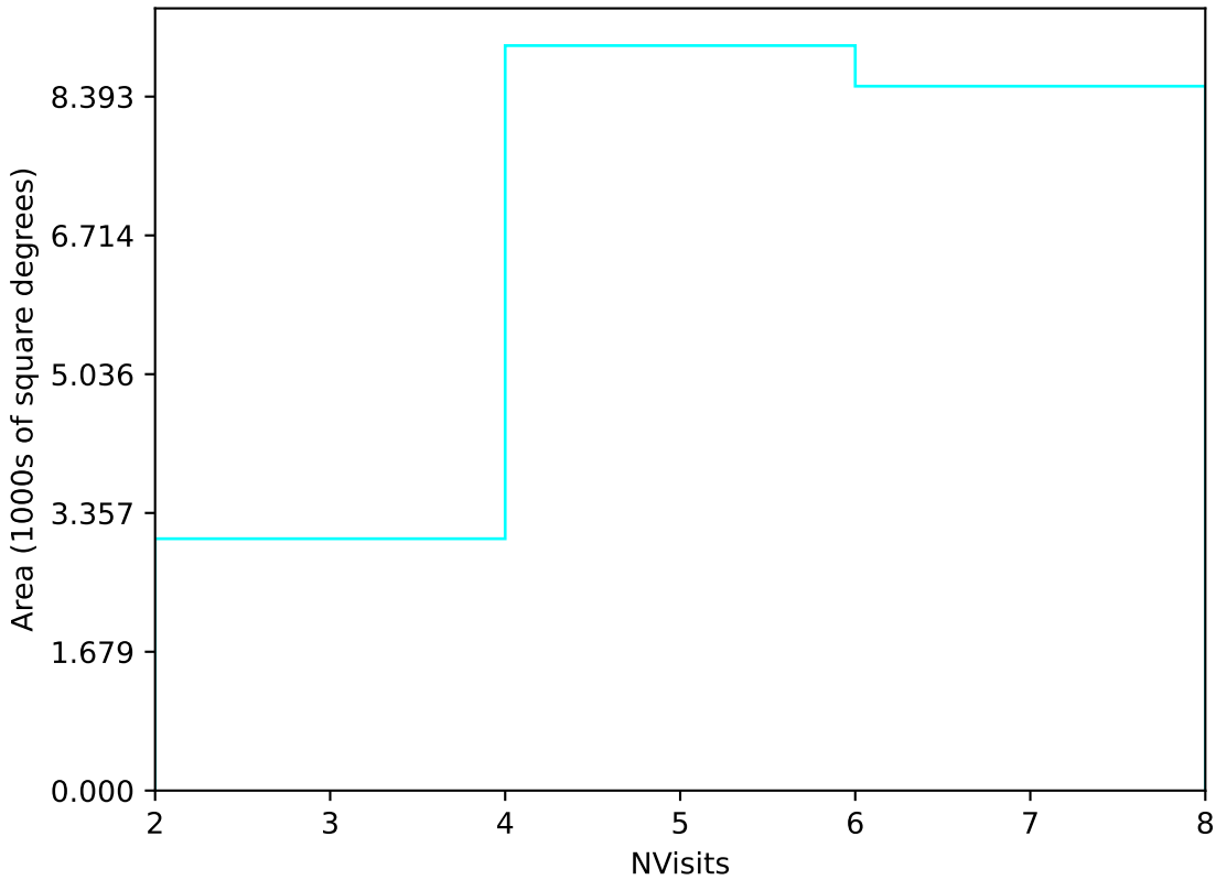
weather_cloudso18v3.4_10yrs Yr 1 u band: NVisits
