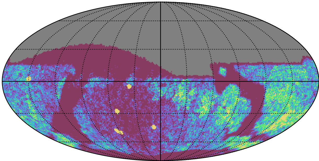
weather_cloudso18v3.4_10yrs Yr 1 r band: NVisits
