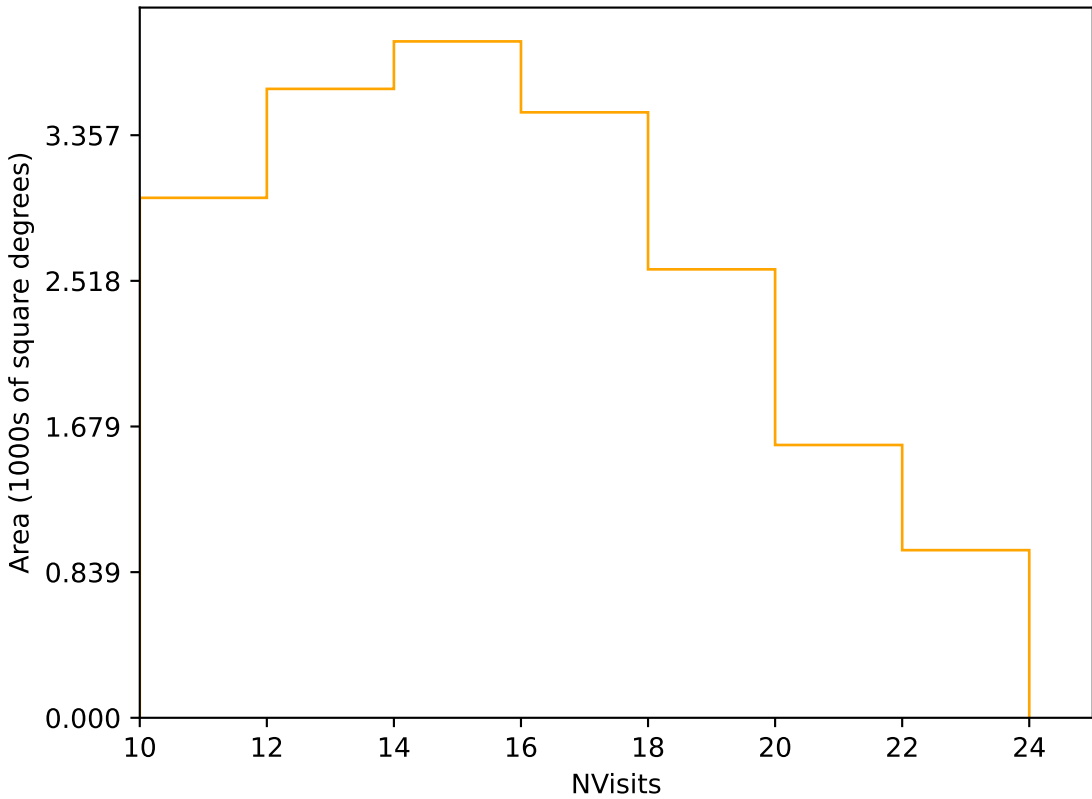
weather_cloudso18v3.4_10yrs Yr 1 r band: NVisits
