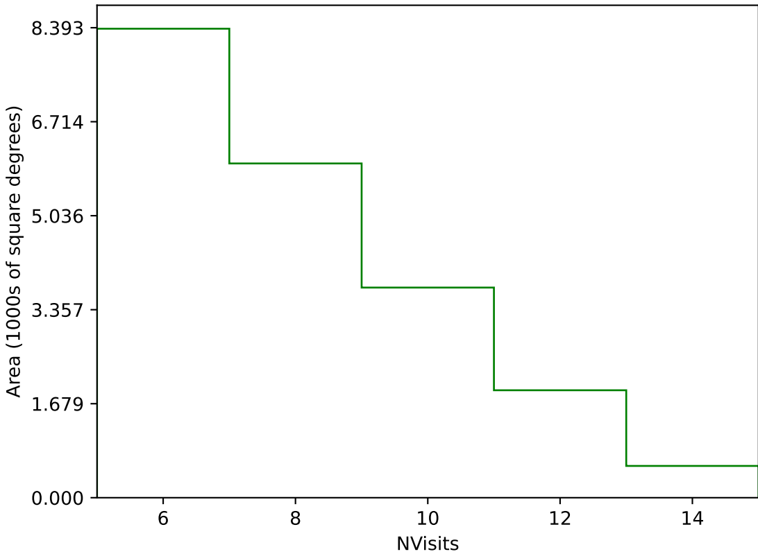
weather_cloudso18v3.4_10yrs Yr 1 g band: NVisits
