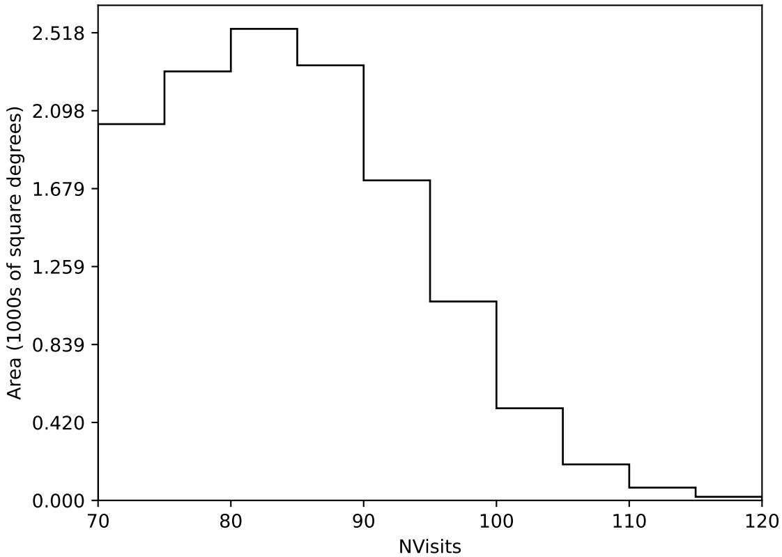
weather_cloudso18v3.4_10yrs Yr 1 all bands: NVisits
