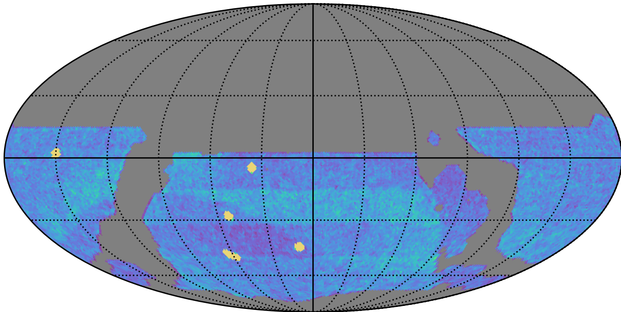
weather_cloudso18v3.4_10yrs WFD all bands: NVisits
