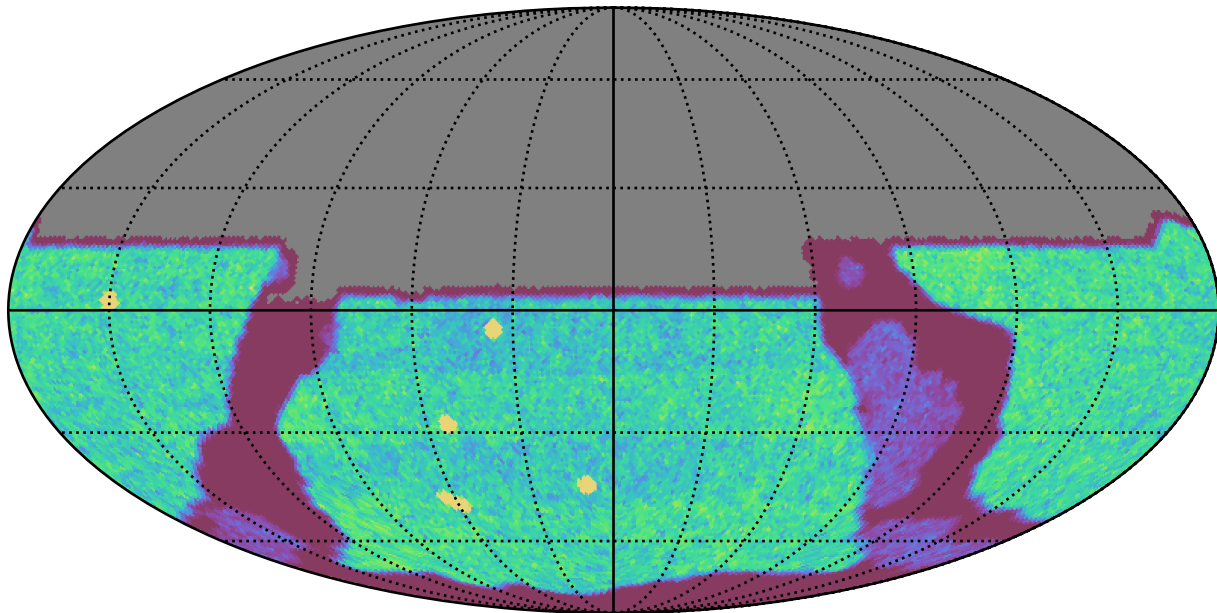
weather_cloudso18v3.4_10yrs All sky u band: NVisits
