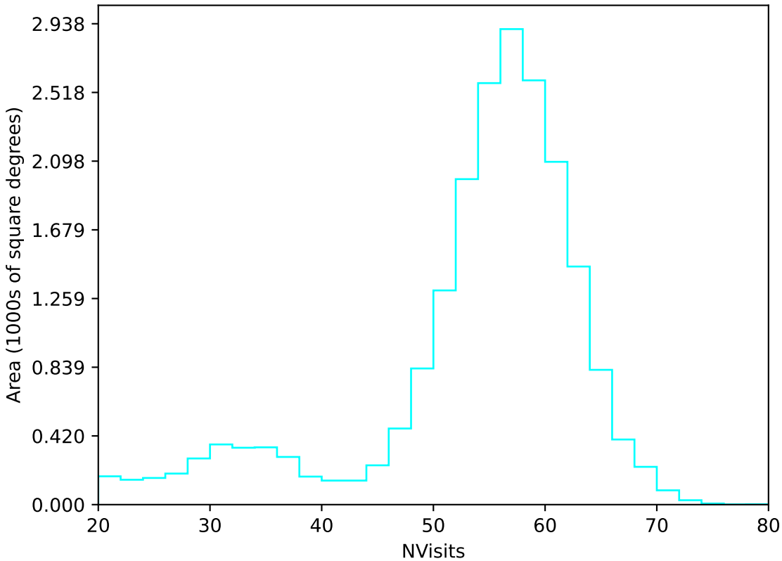
weather_cloudso18v3.4_10yrs All sky u band: NVisits
