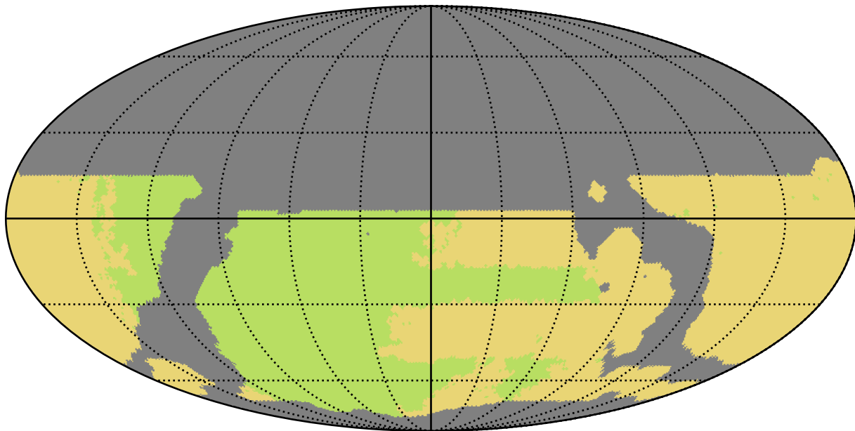
weather_cloudso18v3.4_10yrs WFD all bands: NSeasons
