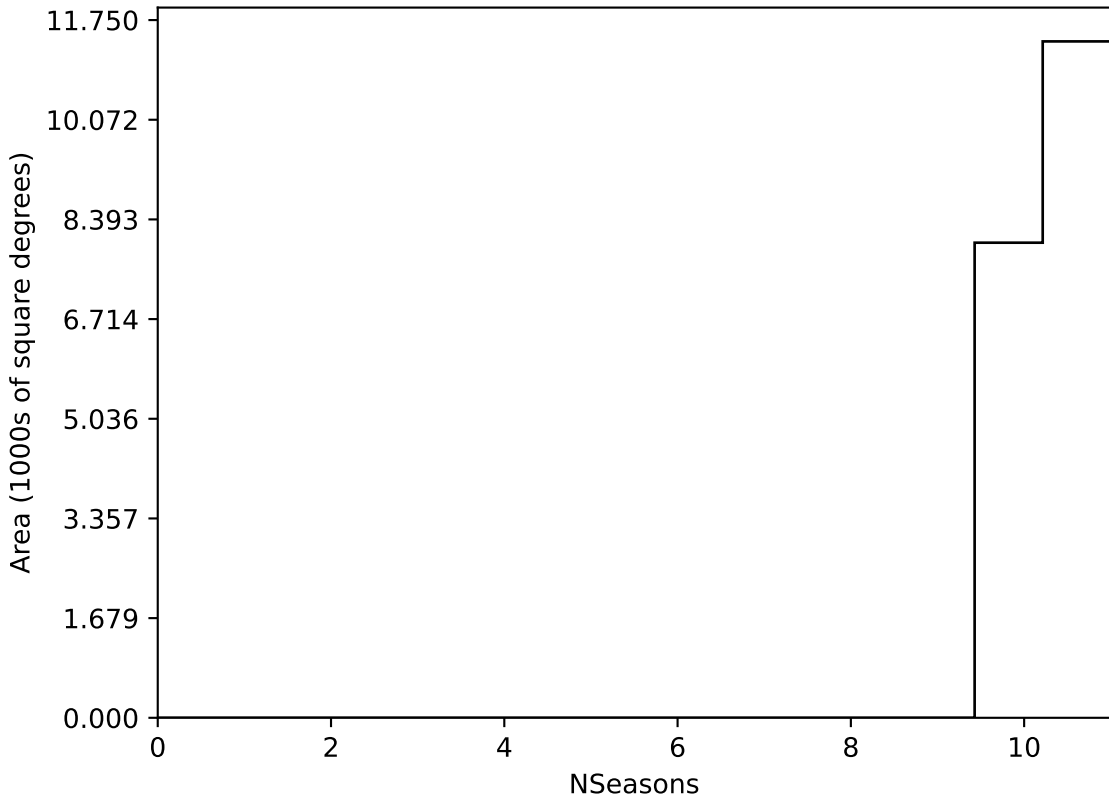
weather_cloudso18v3.4_10yrs WFD all bands: NSeasons
