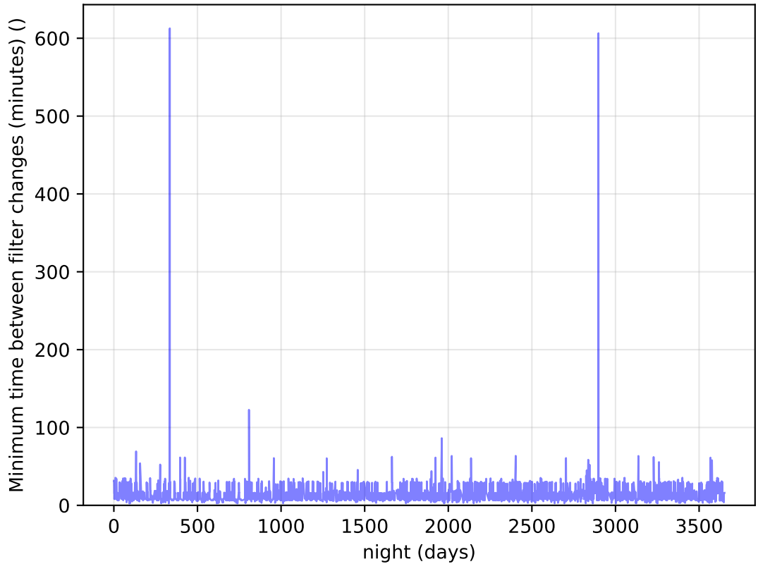
weather_cloudso18v3.4_10yrs Per Night: Minimum time between filter changes (minutes)
