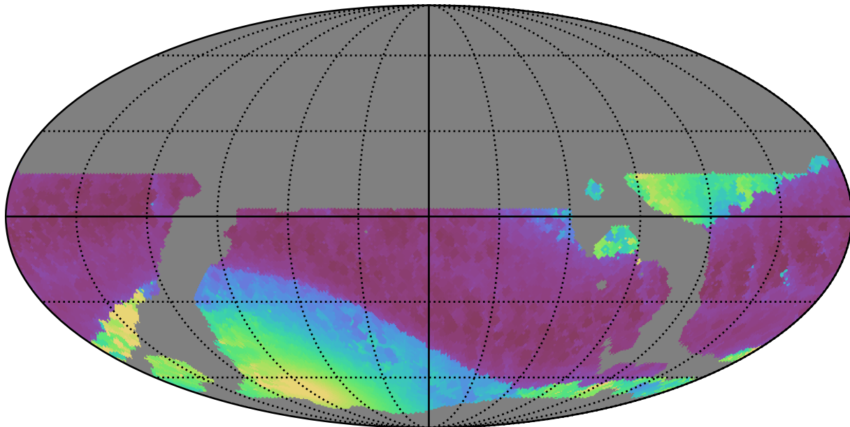
weather_cloudso18v3.4_10yrs WFD all bands: Min solarElong
