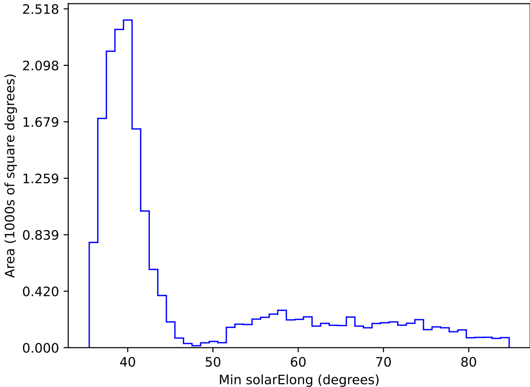
weather_cloudso18v3.4_10yrs WFD all bands: Min solarElong
