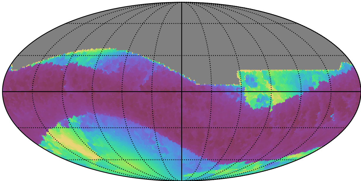
weather_cloudso18v3.4_10yrs All sky all bands: Min solarElong
