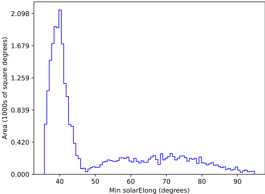
weather_cloudso18v3.4_10yrs All sky all bands: Min solarElong
