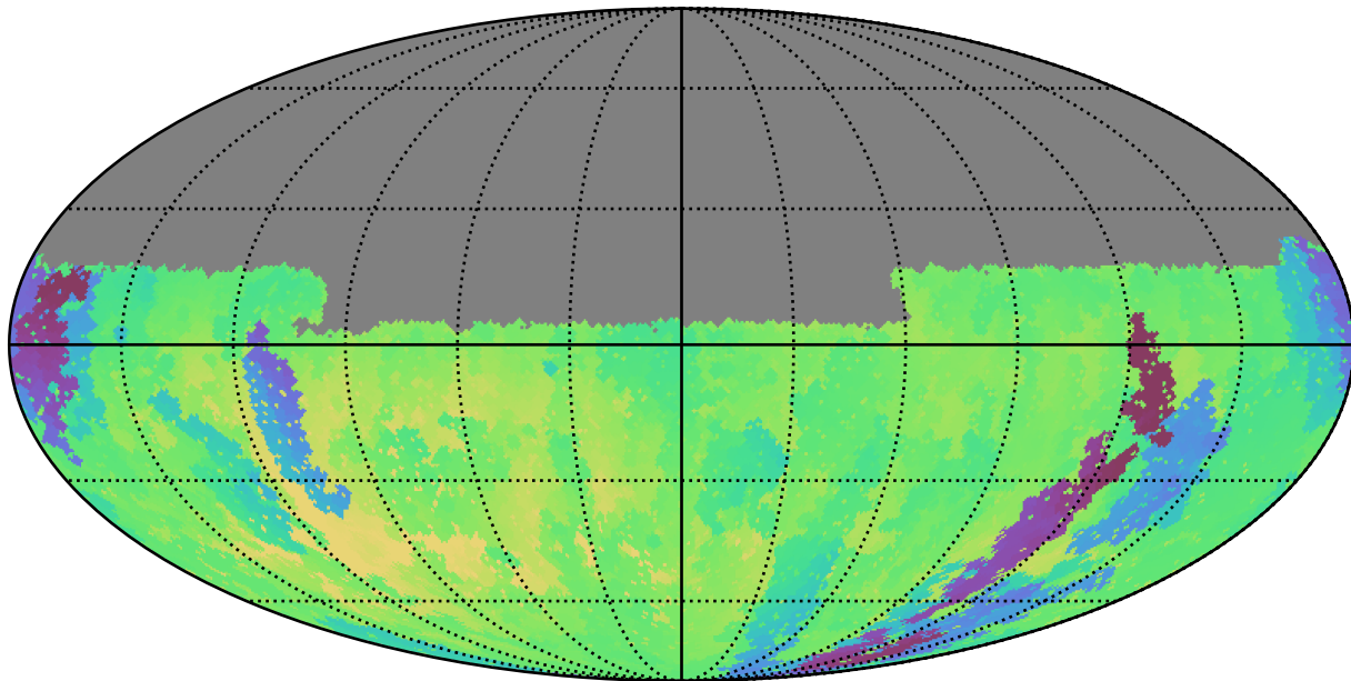
weather_cloudso18v3.4_10yrs Yr 1 u band: Min skyBrightness
