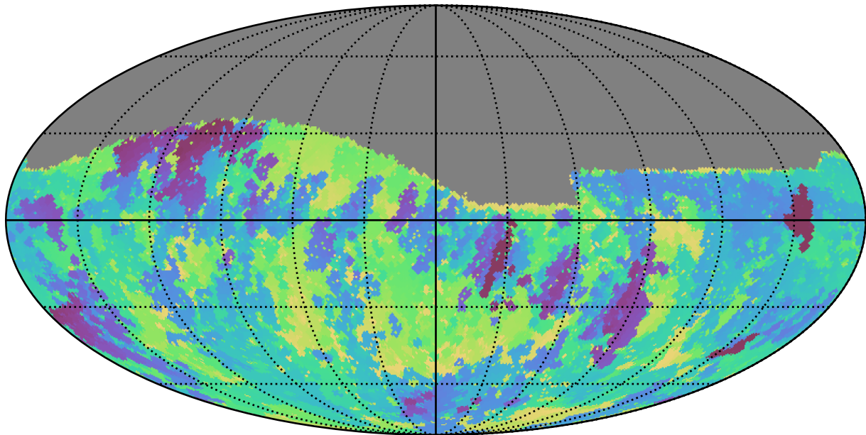
weather_cloudso18v3.4_10yrs Yr 1 r band: Min skyBrightness
