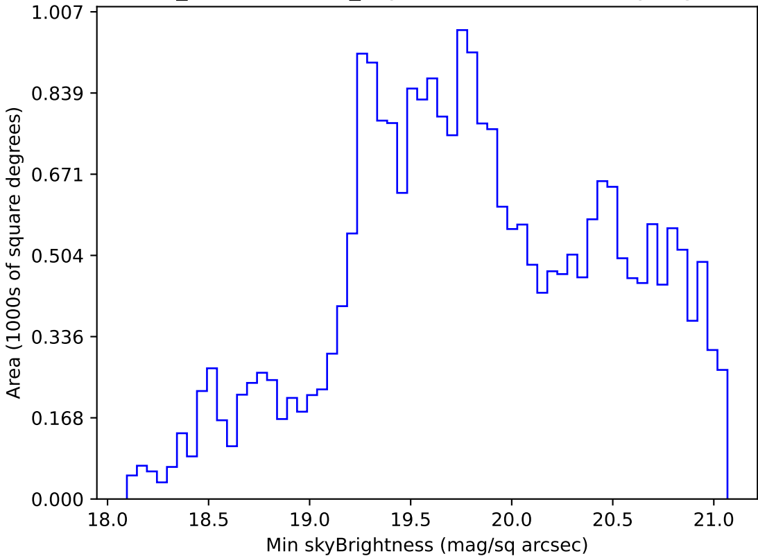
weather_cloudso18v3.4_10yrs Yr 1 r band: Min skyBrightness
