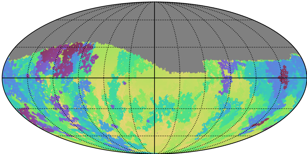
weather_cloudso18v3.4_10yrs Yr 1 g band: Min skyBrightness
