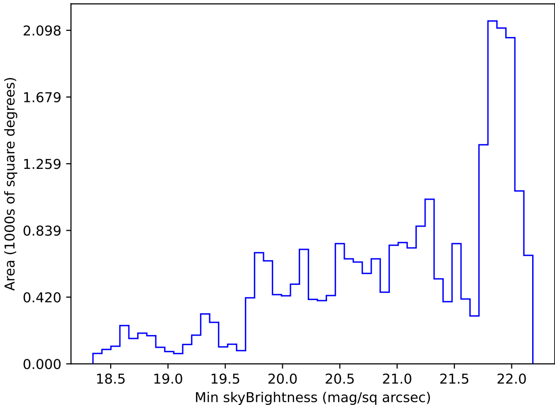
weather_cloudso18v3.4_10yrs Yr 1 g band: Min skyBrightness
