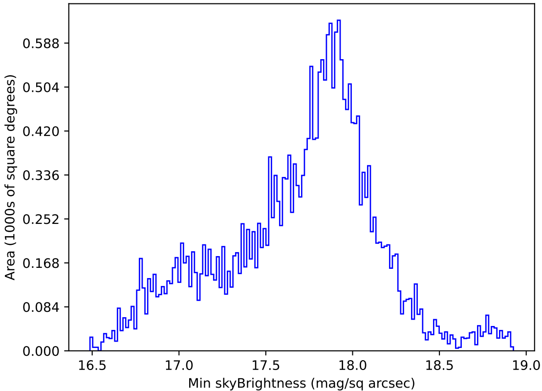
weather_cloudso18v3.4_10yrs Yr 1 all bands: Min skyBrightness
