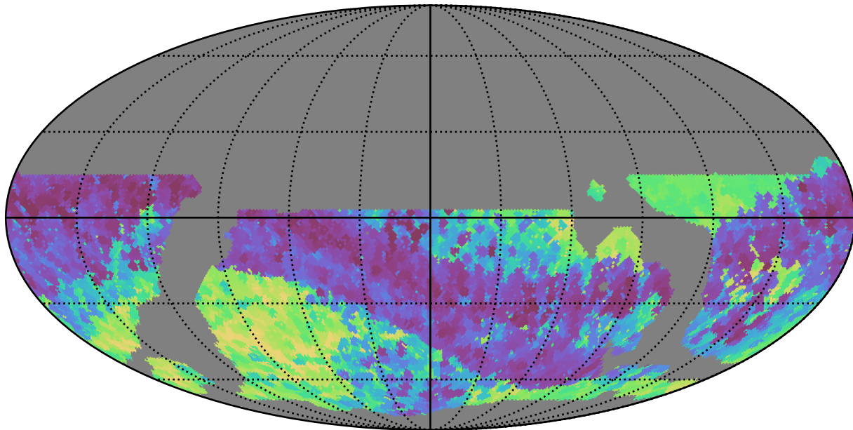
weather_cloudso18v3.4_10yrs WFD z band: Min skyBrightness
