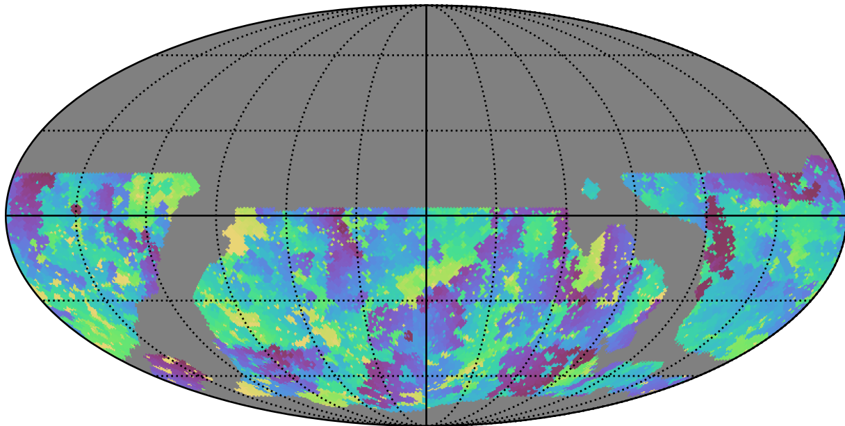
weather_cloudso18v3.4_10yrs WFD u band: Min skyBrightness
