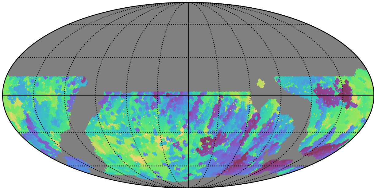
weather_cloudso18v3.4_10yrs WFD r band: Min skyBrightness
