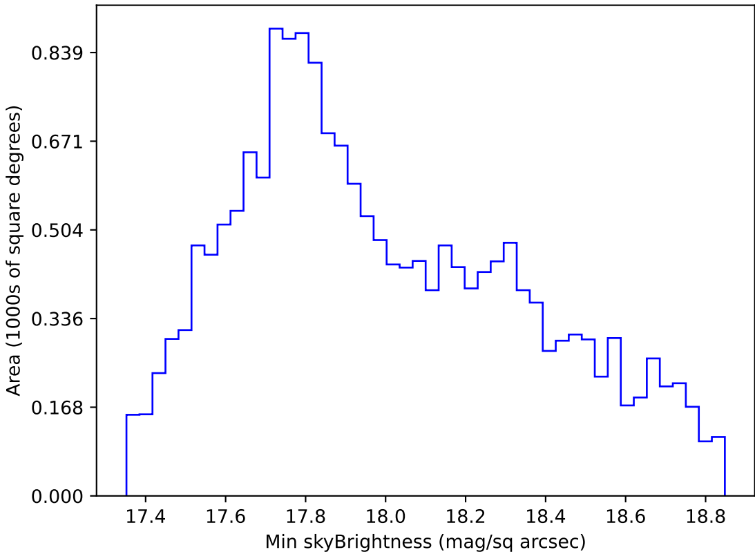
weather_cloudso18v3.4_10yrs WFD i band: Min skyBrightness
