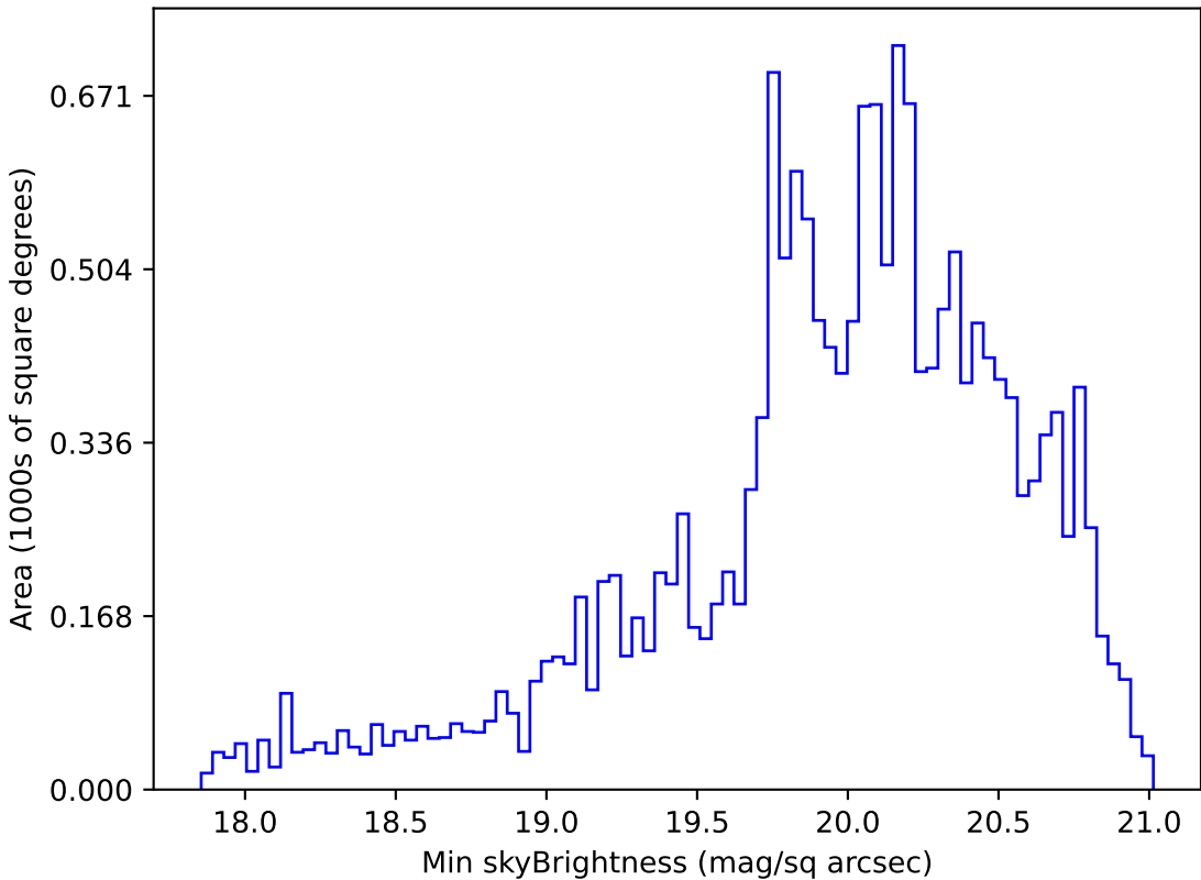
weather_cloudso18v3.4_10yrs WFD g band: Min skyBrightness
