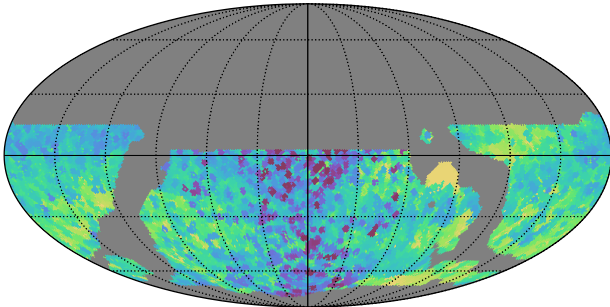
weather_cloudso18v3.4_10yrs WFD all bands: Min skyBrightness
