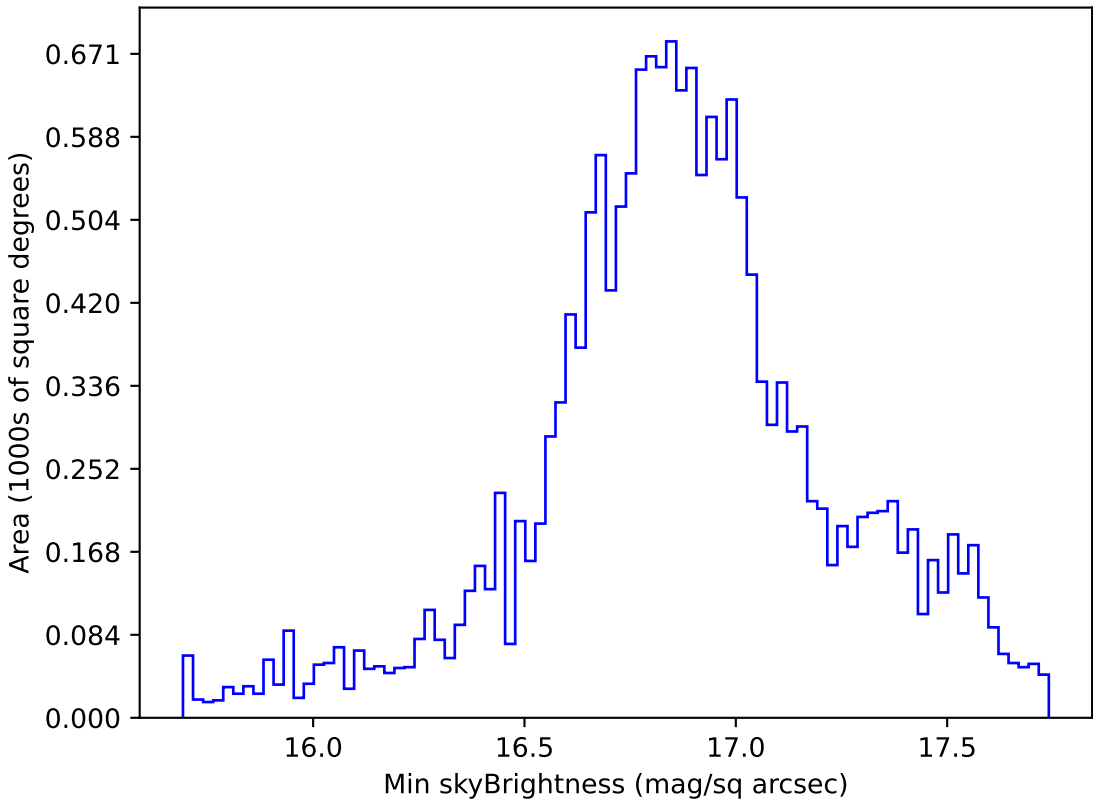
weather_cloudso18v3.4_10yrs WFD all bands: Min skyBrightness
