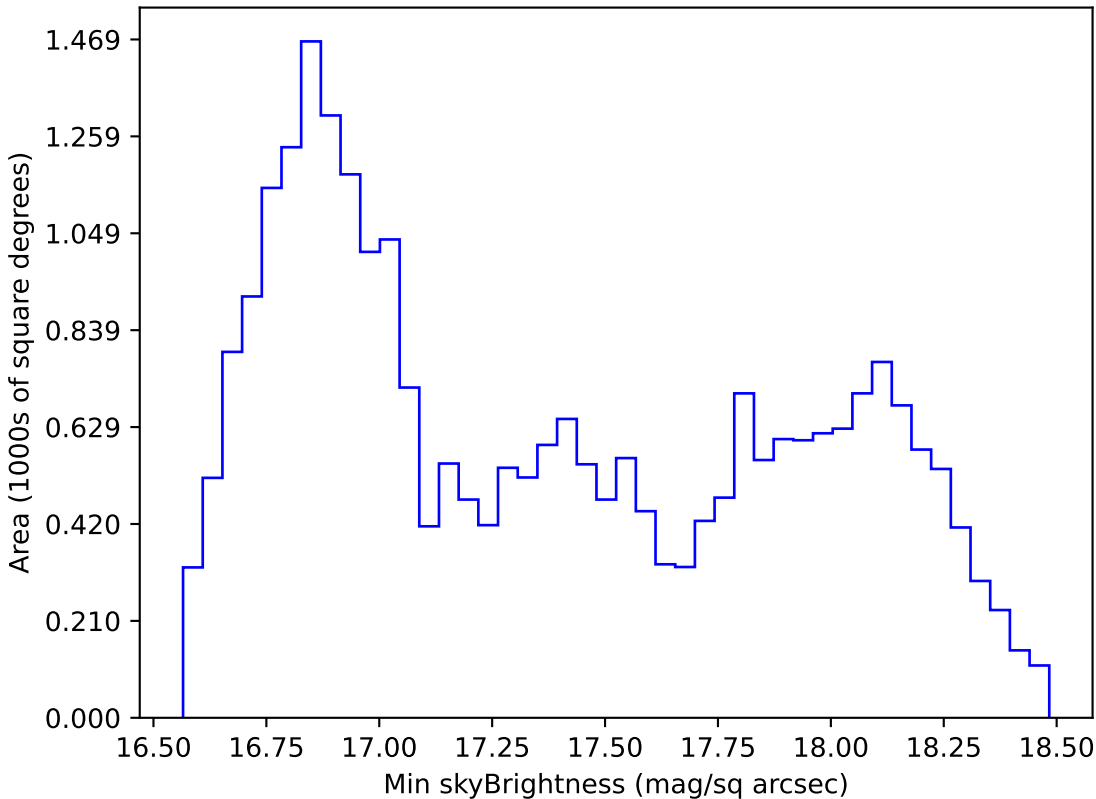
weather_cloudso18v3.4_10yrs All sky z band: Min skyBrightness
