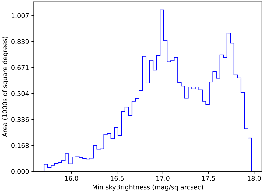
weather_cloudso18v3.4_10yrs All sky y band: Min skyBrightness
