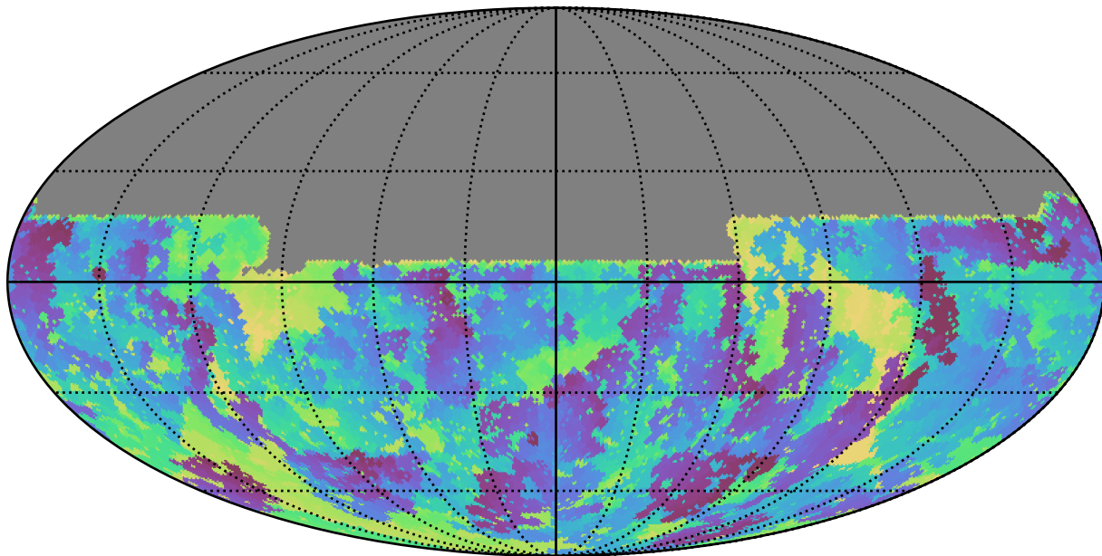
weather_cloudso18v3.4_10yrs All sky u band: Min skyBrightness
