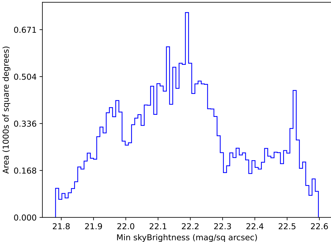
weather_cloudso18v3.4_10yrs All sky u band: Min skyBrightness
