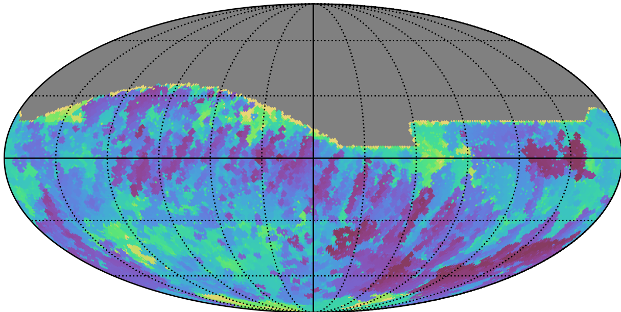
weather_cloudso18v3.4_10yrs All sky r band: Min skyBrightness
