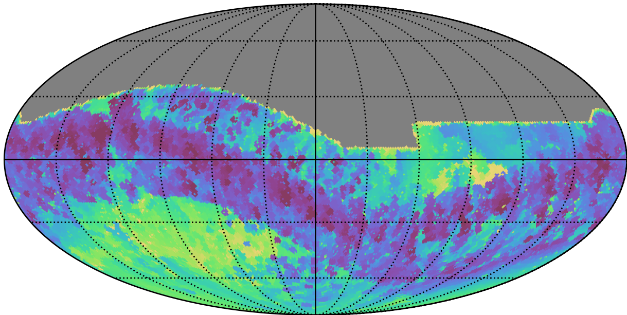
weather_cloudso18v3.4_10yrs All sky i band: Min skyBrightness
