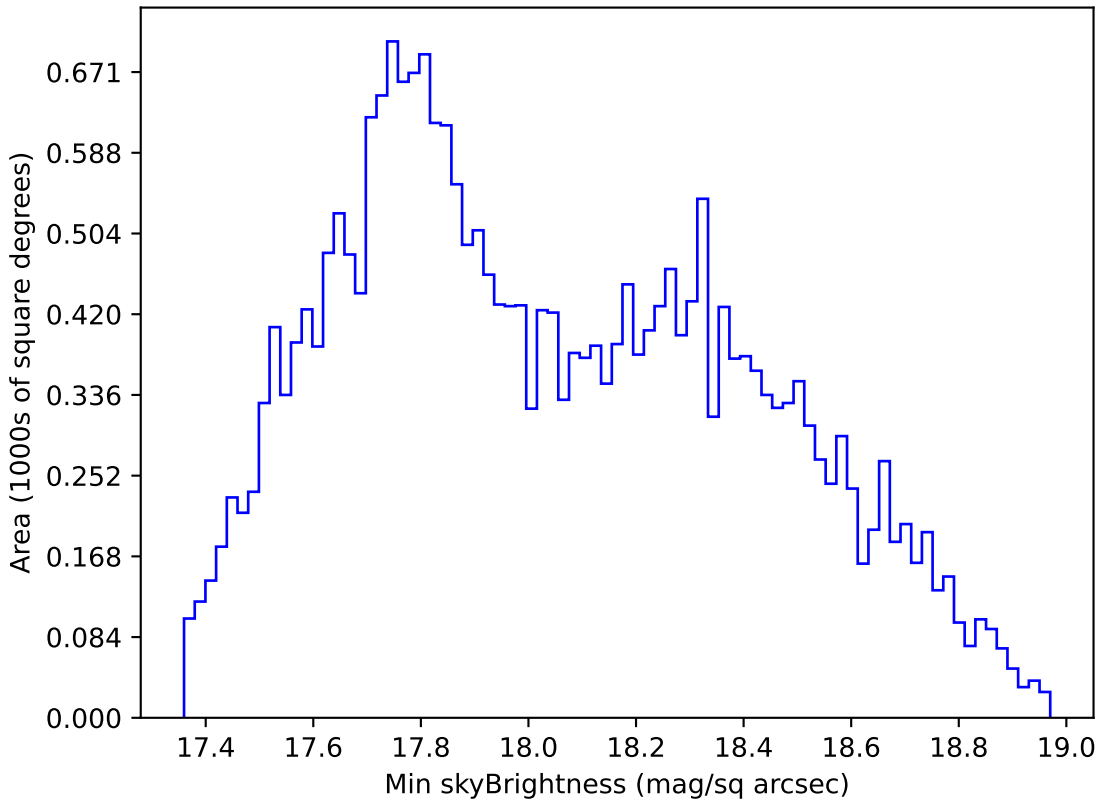
weather_cloudso18v3.4_10yrs All sky i band: Min skyBrightness
