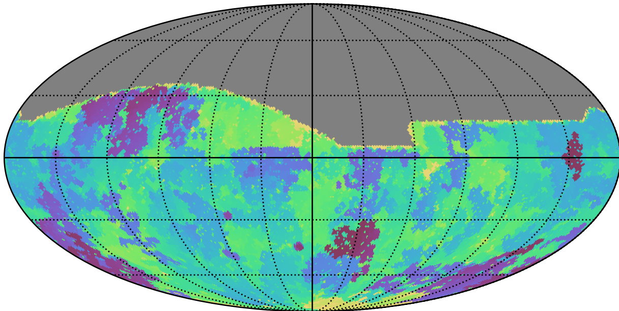
weather_cloudso18v3.4_10yrs All sky g band: Min skyBrightness
